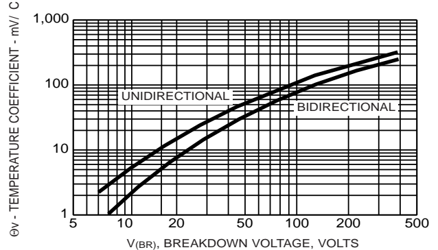
FIG. 12 - BREAKDOWN VOLTAGE TEMPERATURE COEFFICIENT CURVE
