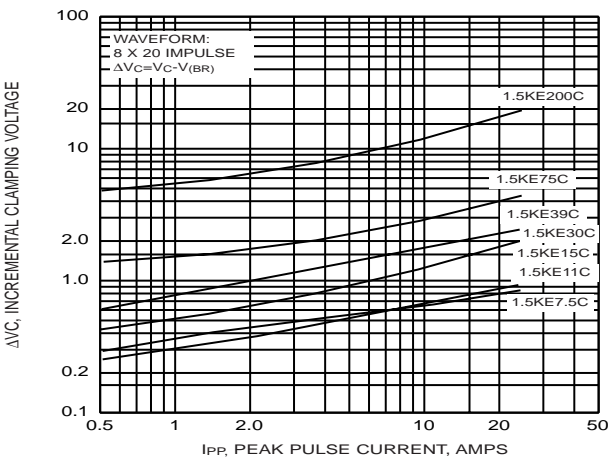
FIG. 9 - INCREMENTAL CLAMPING VOLTAGE CURVE BI-DIRECTIONAL
