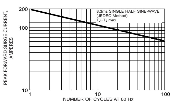
FIG. 6 - MAXIMUM NON-REPETITIVE PEAK FORWARD SURGE CURRENT UNI-DIRECTIONAL ONLY
