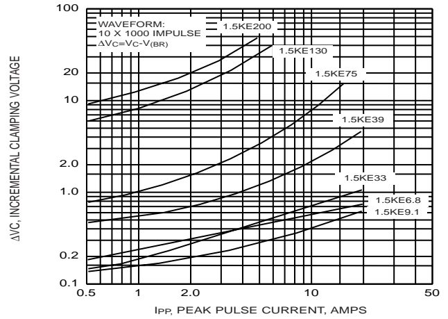
FIG. 8 - INCREMENTAL CLAMPING VOLTAGE CURVE UNI-DIRECTIONAL
