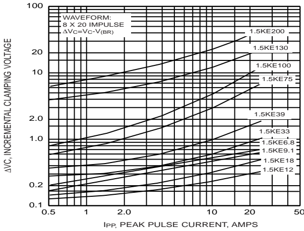
FIG. 7 - INCREMENTAL CLAMPING VOLTAGE CURVE UNI-DIRECTIONAL
