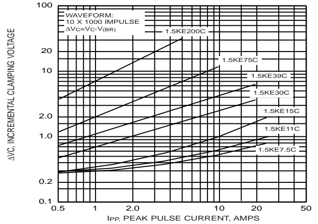
FIG. 10 - INCREMENTAL CLAMPING VOLTAGE CURVE BI-DIRECTIONAL
