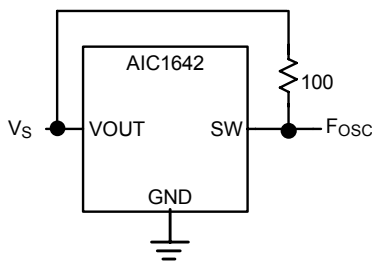
Fig. 3 Test Circuit 3
