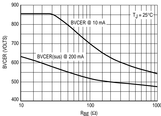
Figure 10. Resistive Breakdown
