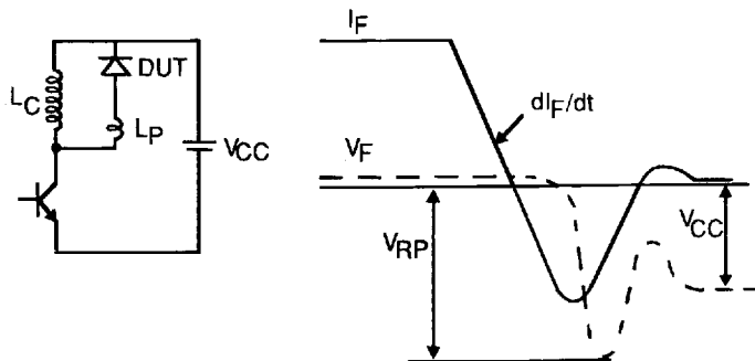
Figure 11 : Turn-off switching characteristics (without series inductance).
