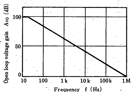
Open loop voltage gain—Frequency Characteristics
