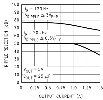
Ripple Rejection vs Output Current (LM1086-5)
