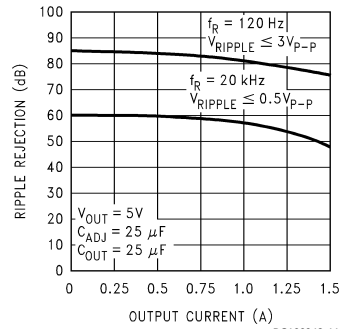
Ripple Rejection vs Output Current (LM1086-Adj.)
