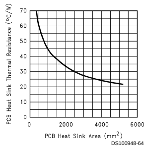
FIGURE 7. Heat sink thermal Resistance vs Area
