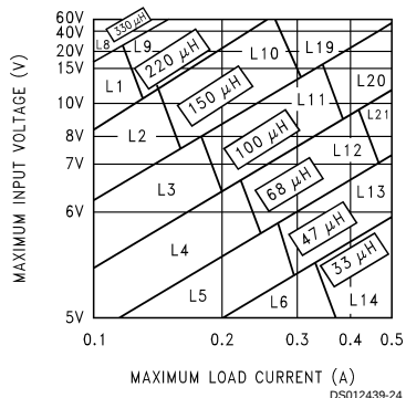
FIGURE 4. LM2594/LM2594HV-3.3
