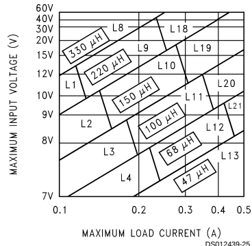
FIGURE 5. LM2594/LM2594HV-5.0
