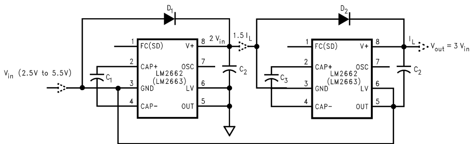
FIGURE 7. Generating +3V_{in} from +V_{in}
