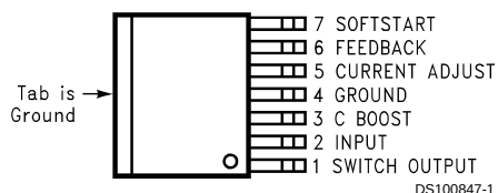
TO-263 Package Top View
