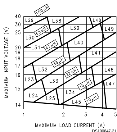
FIGURE 5. LM2679-12
