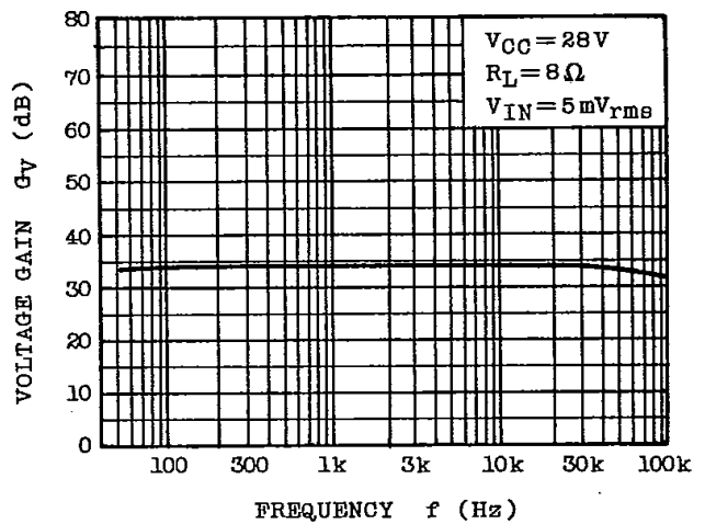
G_V - f
