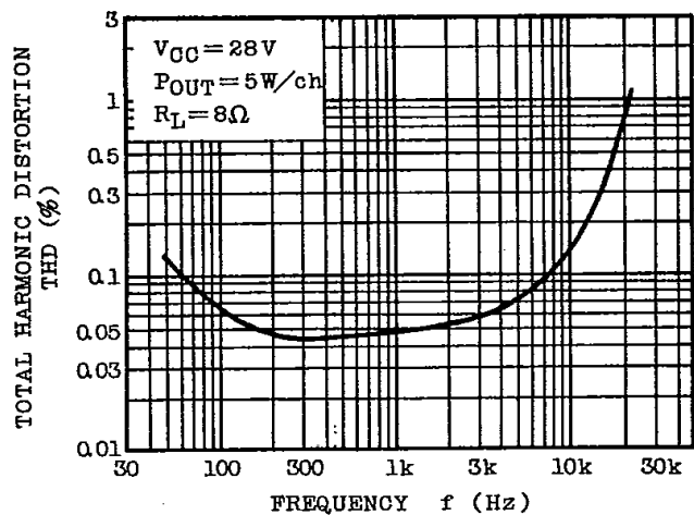
THD - f
