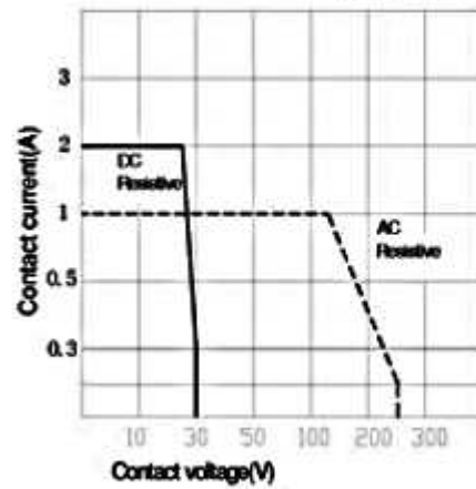
Contact Switching Capacity
