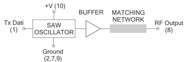
Block diagram
